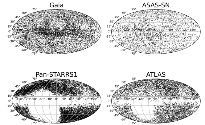
Fig. 13. Survey coverage for GSA ( top-left ), compared to three other transient surveys: ASAS-SN ( top-right ), ATLAS ( bottom-right ) and PanSTARRS1 ( bottom-left ). Data are presented in Galactic coordinates, with the centre of the Galaxy at the centre of each figure. Transients were all compiled using our local database as described in Sect. 2.8, and reported during the date range June 11 2016 to December 31 2019 inclusive.
