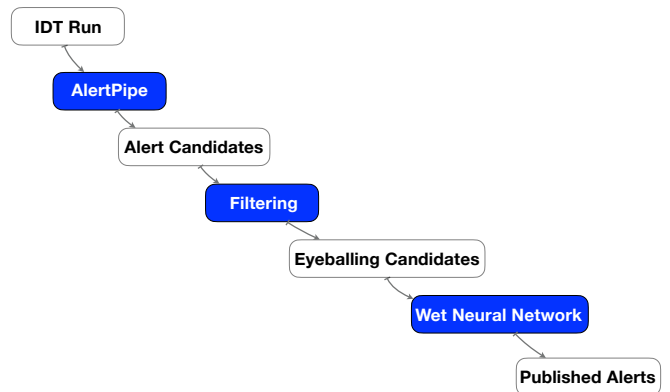
Fig. 3. Schematic of the data flow and processing performed by the GSA project. Unfilled boxes indicate data, blue boxes (dark grey) show processes. Wet Neural Network refers to the eyeballing, voting and commenting process performed by humans.
