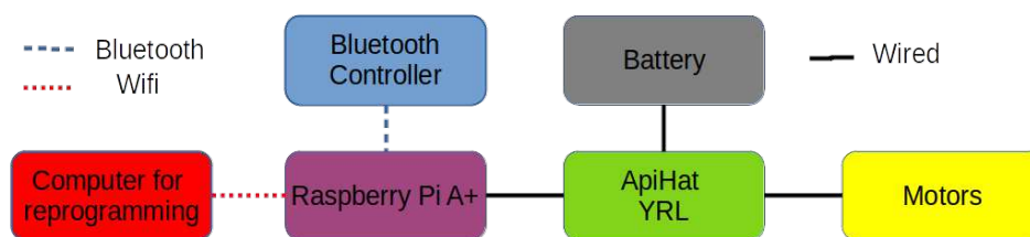
Figure 2. Block diagram of electronic components.
