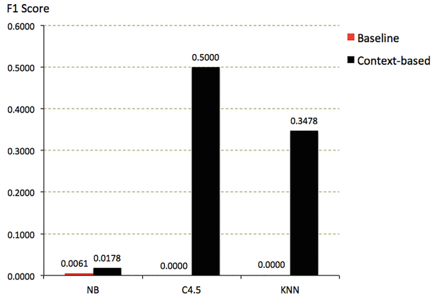
Fig. 6. F1 scores obtained by different classification models with Data2. These are averages summarized from 20 trials of 10-fold cross validation.
