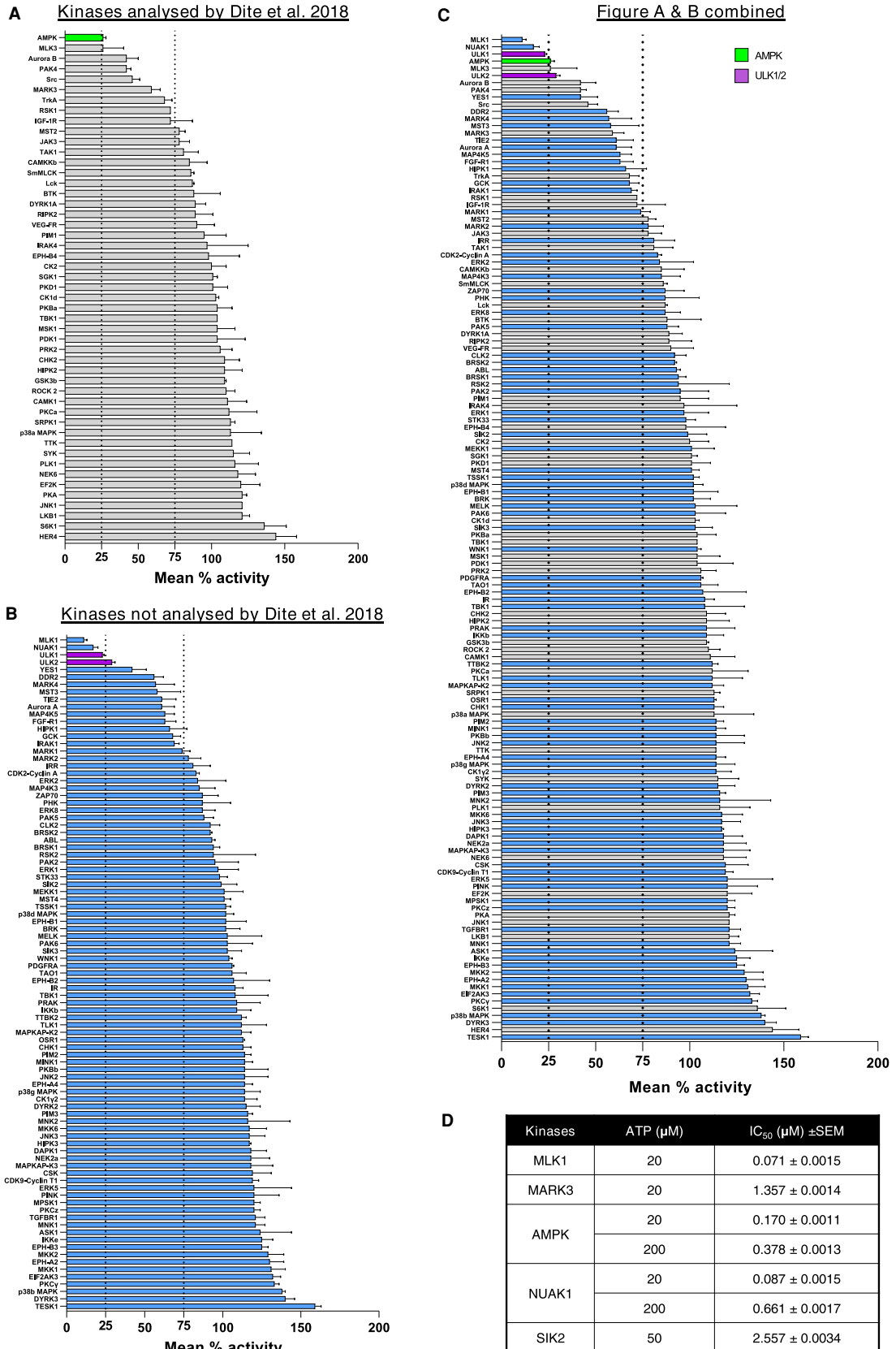
Figure 5. Kinase selectivity profile for SBI-0206965.
