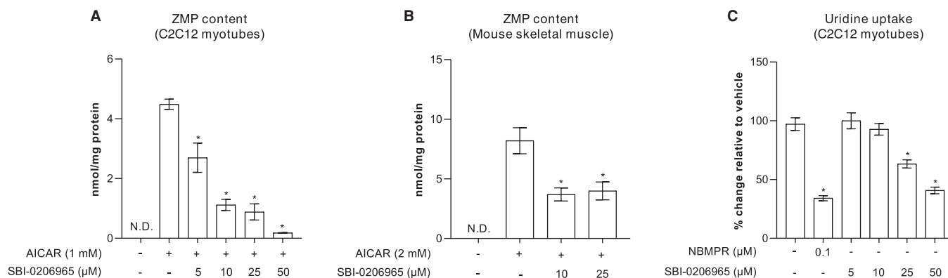
Figure 4. SBI-0206965 inhibits AICAR and uridine uptake in C2C12 myotubes.
