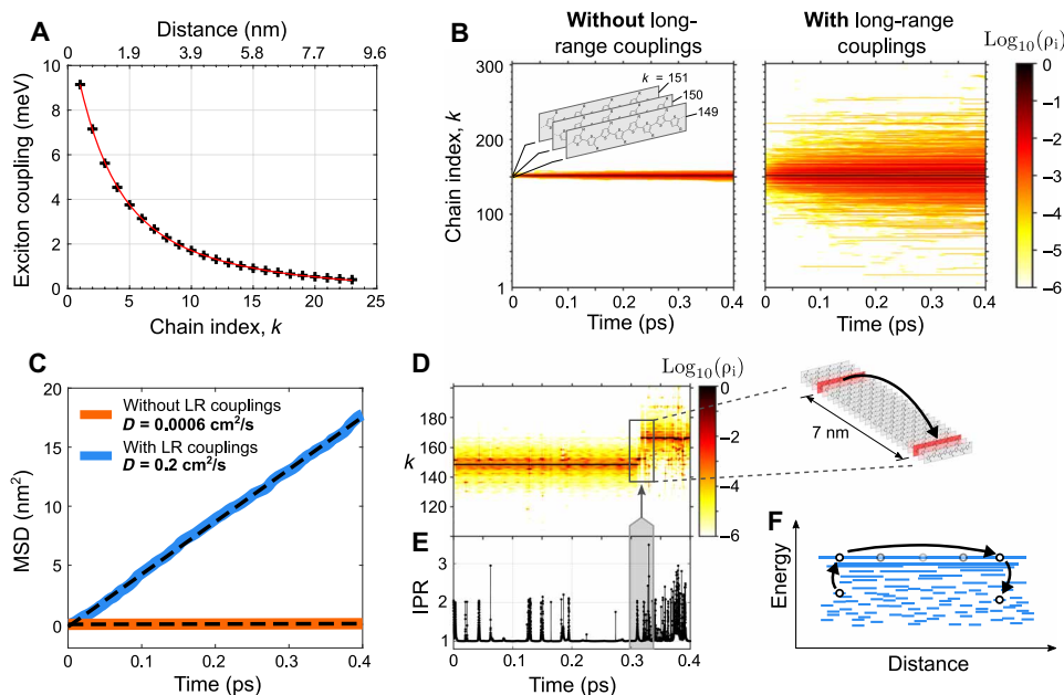
Fig. 4. Simulations of exciton diffusion. (A) INDO/SCI (intermediate neglect of differential overlap/single configuration interaction) calculations of the Coulombic exciton couplings in a 24-chain stack, with a biexponential fit. (B) Sum of many individual surface hopping simulations of exciton diffusion in a 1D stack (i.e., trajectories) with and without long-range (LR) exciton couplings. The color scale indicates the log of the normalized total exciton density. (C) Associated MSD derived from (B). The MSD evolves linearly, indicating that an equilibrium regime is reached. Linear fits (dashed) give diffusion constants of D = 0.22 \text{ cm}^2/\text{s} and 6 \times 10^{-4} \text{ cm}^2/\text{s} with and without the inclusion of long-range exciton couplings, respectively, which demonstrates how long-range couplings markedly increase diffusion. (D) Exciton density over a single representative trajectory, with (E) the associated IPR. The IPR remains mostly low ( \sim 1 ), indicating that the exciton is mostly localized on a single chain, but occasionally (as indicated in the highlighted region), the IPR increases as the exciton transiently occupies higher-energy delocalized states, and when it does, the exciton tends to move large distances by “surfing” along the EDOS as shown by the inset. (F) Schematic illustrating how excitons can transiently occupy high-energy delocalized states to move large distances. These delocalized states are responsible for the majority of the diffusion, a fact that is emphasized by making the comparison to the case of no long-range couplings, where no such delocalized states are occupied, and the diffusion is severely restricted.
