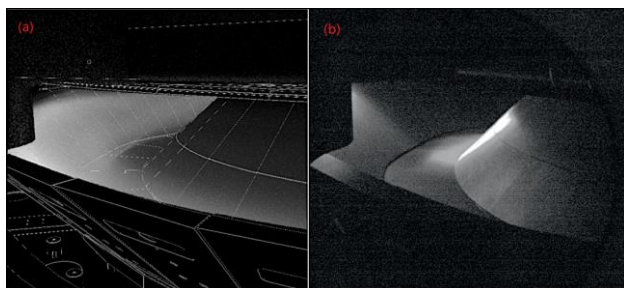
FIG. 8. (a) Modelled divertor plasma view by CHERAB. (b) Actual divertor view illuminated by flash lamp.
