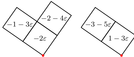
FIGURE 3. A semistandard tableau \mathbb{S} \in \text{SStd}_{(3;4,0)}(((1^2), (2, 1)), (\emptyset, (2, 1^3))) . We have tilted the components of this 2-partition \varepsilon units anti-clockwise so that the x -coordinate of a box (r, c, m) is equal to \text{ct}(r, c, m) - m/\ell - (r + c)\varepsilon . Two possible corresponding basis elements for this tableau are depicted in Figure 15.
