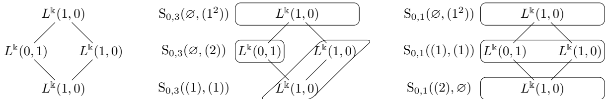
FIGURE 22. The projective cover of the irreducible module L^k(1,0) and its 2 distinct cell-filtrations. As both n and \ell increase, we obtain many more distinct filtrations on each projective module.
