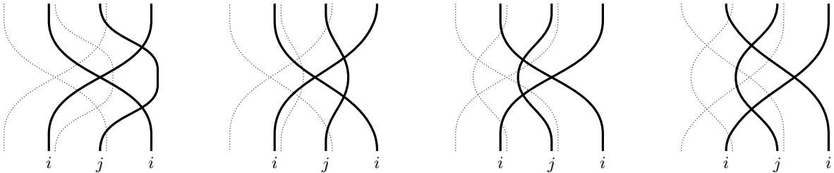
FIGURE 19. The wider diagrams A \in E_\omega^\sigma \mathbb{A}_n^{\mathbb{k}}(\sigma) E_\omega^\sigma containing a triple-crossing of the form depicted in Figure 18. The first and final of which are already of the required form.
