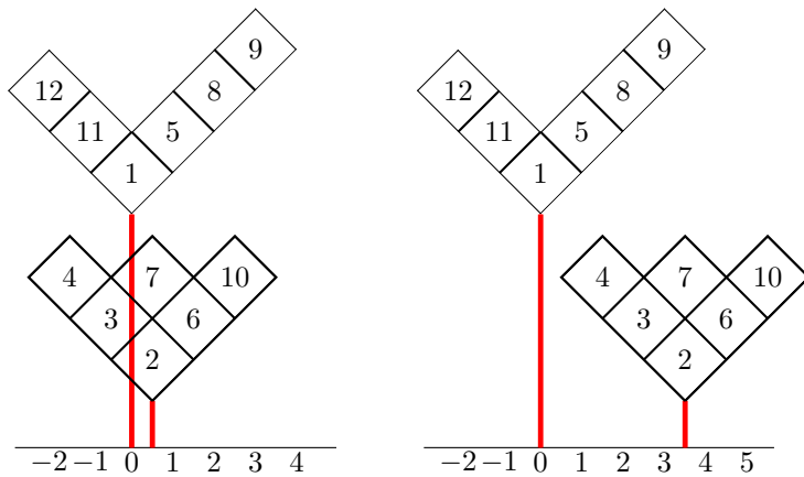
FIGURE 2. Tableaux \mathfrak{s} \in \text{Std}_{(3;0,1)}(\lambda) and \mathfrak{t} \in \text{Std}_{(3;0,4)}(\lambda) for \lambda = ((4, 1^2), (3, 2, 1)) .
