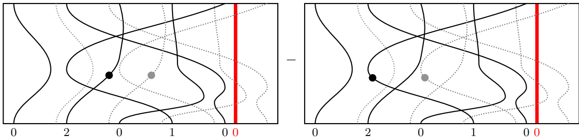
FIGURE 6. Undoing the double-crossing of the ghost 1-strand and a solid 2-strand in the rightmost diagram of Figure 5 using relation (A6)
