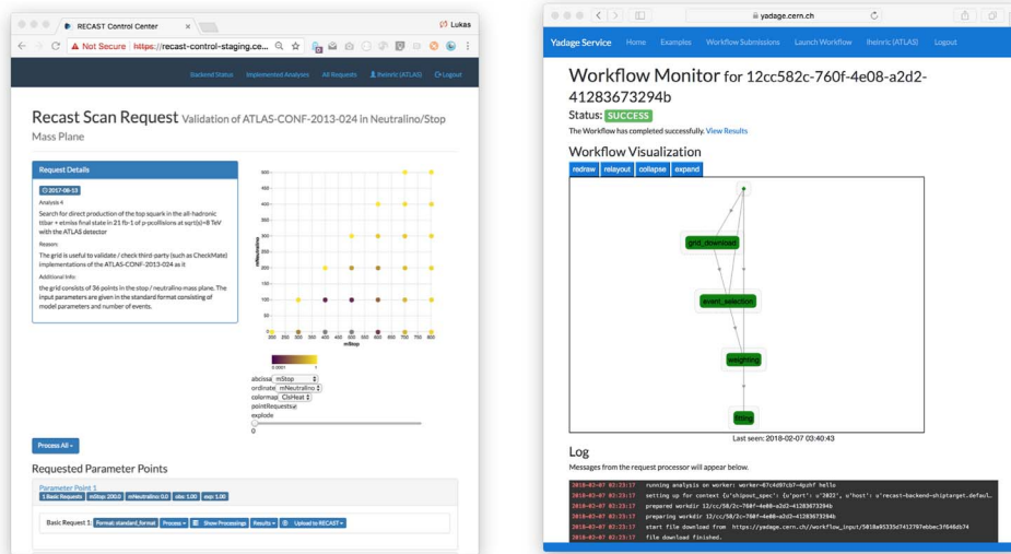
Figure 83. Left: web-based interface for the RECAST back end for an experiment that presents the requested parameter points and color-coded results. Right: an experiment-internal reinterpretation executing on the distributed infrastructure built by CAP and RECAST.
