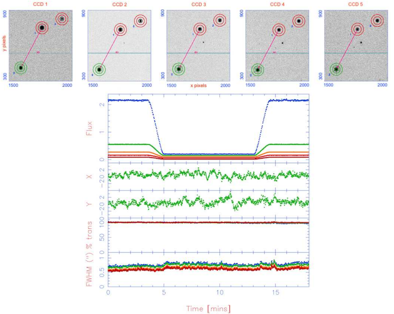
Figure 9. A screenshot of the HiPERCAM data-reduction pipeline. Top panel: Zoomed-in images in u_s g_s r_s i_s z_s of the target (the eclipsing red-dwarf/white-dwarf binary NN Ser) and two comparison stars, surrounded by software apertures defining the object and sky regions. Aperture 1 is the target, and apertures 2 and 3 are the comparison stars. Aperture 2 is green because it has been defined as the reference star for centroiding. The pink arrows show that the target and reference apertures are linked, so that the positional offset between the two is held constant when the target almost disappears during eclipse. Bottom panel: From top to bottom, the target flux divided by the comparison star flux in u_s g_s r_s i_s z_s (each with a flux offset of 0.05 added to separate the light curves during eclipse minimum), the comparison star x and y positions, the sky transparency measured from the comparison star flux, and the seeing measured from the comparison-star FWHM in u_s g_s r_s i_s z_s .
