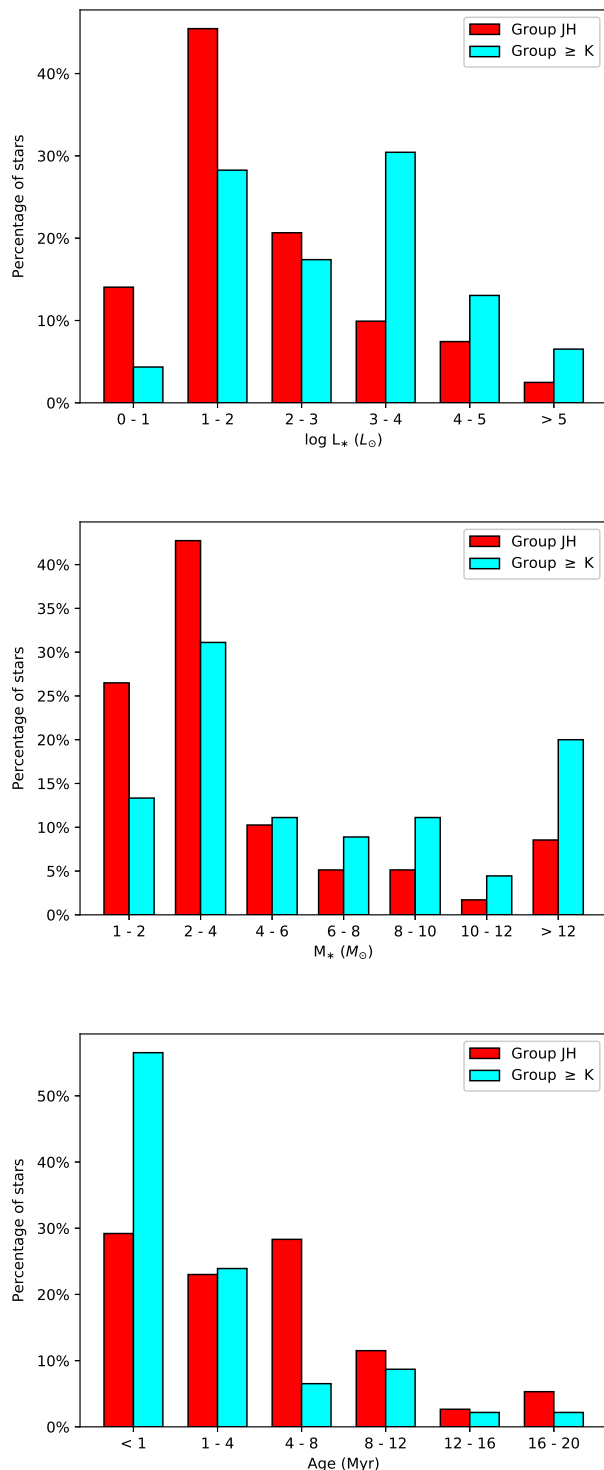
Fig. 6: Histogram comparing the distributions of stellar parameters (luminosity, stellar mass, and age) and JHK groups, as indicated in the x-axis and the legend.
