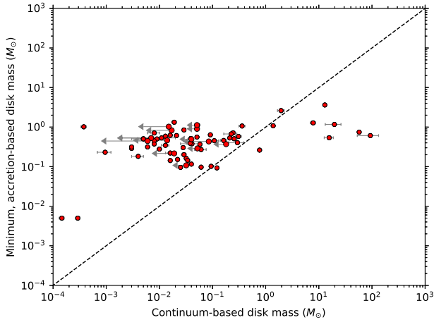
Fig. 2: Disk masses from accretion and age vs. those from dust emission at millimeter wavelengths. Upper limits are represented by arrows. The dashed black line indicates equal values.
