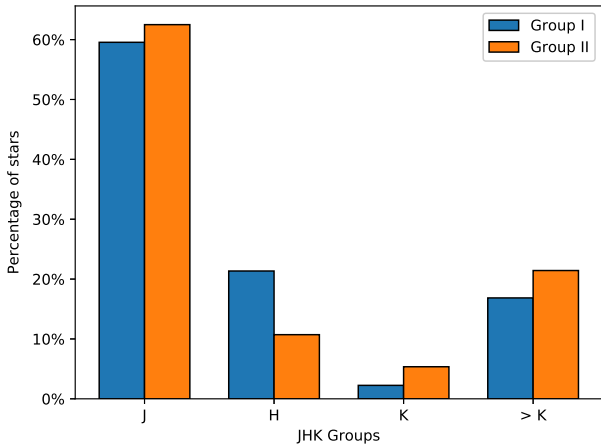
Fig. 4: Histogram comparing the distributions of the JHK groups (based on the wavelength at which the infrared excess starts) and M01 groups (based on the shape of the SEDs), as indicated in the x-axis and the legend.
