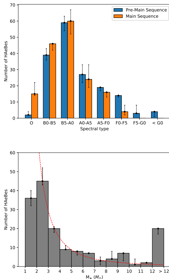
Fig. 3: Top panel: Current distribution of spectral types in the PMS and expected distribution when the stars reach the MS, as indicated in the legend. The error bars reflect the uncertainties on the spectral types. Bottom panel: Number of HAeBes vs. stellar mass. The error bars for the number of stars per bin considering the uncertainties in M_{*} are indicated. The dashed red line corresponds to the IMF (Salpeter 1955) normalized to the bin 2-3 M_{\odot} . Stars with masses > 12 M_{\odot} have been grouped together for simplicity.
