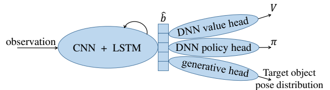
Fig. 4. NN architecture.
