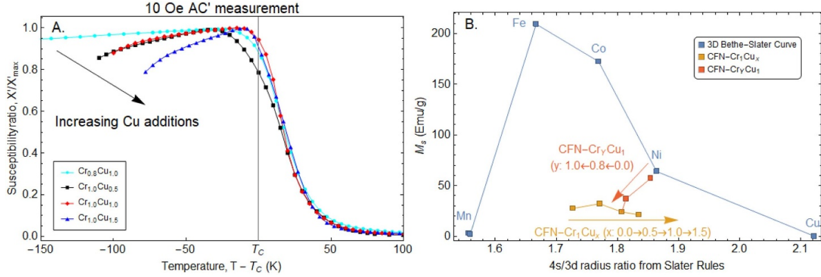
Figure 9. (a) AC measurements ( X' ) of CFN-Cr 1.0 Cu x and CFN-Cr 0.8 Cu 1.0 sample with T_C < 300 K. For easier comparison, the data has been scaled against respective T_C values on the x -axis and respective X'_{\max} values on the y -axis. (b) Position of the CoFeNi-Cr y Cu x compositions with respect to a reconstructed Bethe–Slater curve using Slater rules [39].
