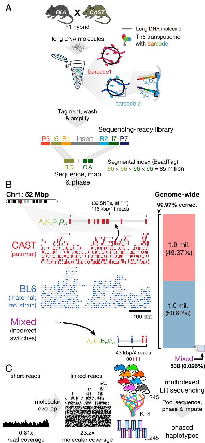
Fig. 1. Haplotyping enables population-scale LR sequencing. (A) Principles of haplotyping. Microbeads coated with barcoded transposon adaptors enable simultaneous molecular barcoding and Tn5-mediated fragmentation of long DNA molecules into sequencing-ready libraries after PCR amplification, all in a single tube. This technique takes advantage of the tendency of DNA to interact only with a single bead in solution ( Inset ). A key feature of haplotyping is that each bead is uniformly coated with a single segmental barcode combination (“beadTag”) made up of four segments of 96 barcodes each (designated “B,” “D,” olive and “C,” “A,” green at the standard i5/i7 index positions of the Illumina Nextera design). Across beads, the four segments represent up to 96^4 or 85 million beadTags. Thus, DNA molecules wrapped around a single bead can be reconstructed from individual short reads that share the same beadTag. (B) Haplotyping in an F1 hybrid mouse between the reference strain C57BL/6 (BL6) and CAST/EiJ (CAST), with detailed view at Chr1: 52 to 52.5 Mbp. Each molecule is represented by a gray
