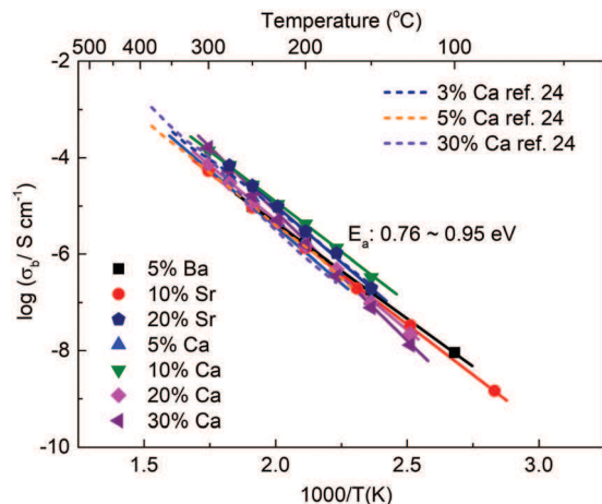
Fig. 2 Arrhenius plot of \sigma_b for N_2 annealed Ba/Sr/Ca-doped BF ceramics with Ca-doped BF data from ref. 24.
