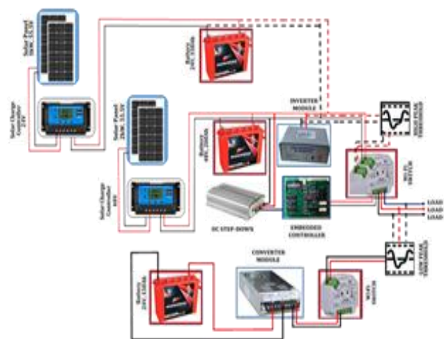
FIGURE 1. Schematic diagram of the IoT based smart energy management system for VPP
