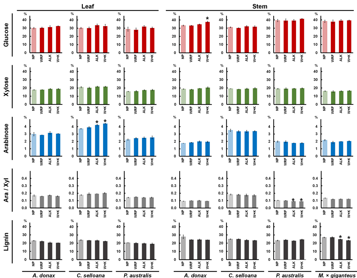
FIGURE 6 | Mean percentage (%) composition of alcohol insoluble residues (AIR) prepared from previously pretreated biomass from Arundo donax , Cortaderia selloana , Phragmites australis and Miscanthus × giganteus (no results are shown for M. × giganteus leaves due to sample losses). Pretreatment acronyms: NP, non-pretreated control samples (incubated only with water; striped bars); WRF, samples pretreated only with Pleurotus ostreatus ; ALK, samples pretreated only with 0.1 M NaOH for 24 h at 21°C; W + K, samples pretreated with P. ostreatus followed by 0.1 M NaOH for 24 h at 21°C. Ara/Xyl is the ratio of arabinose to xylose determined in the biomasses. Pairwise t -tests were performed between each treatment and control (NP) samples to evaluate the impact of the pretreatments in relation to NP samples for each variable, the treatments which are significantly different from the NP controls are marked with a *** ( p \leq 0.05 ). Error bars represent the standard error of the sample replicates.
