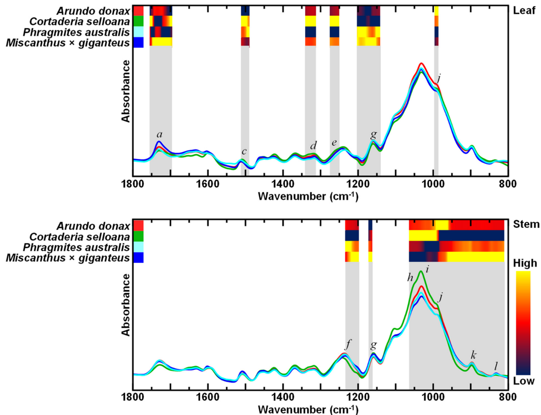
FIGURE 2 | Attenuated total reflectance Fourier transform mid-infrared (FTIR-ATR) spectra of alcohol insoluble residue (AIR) of leaf and stem biomass from Arundo donax , Cortaderia selloana , Phragmites australis and Miscanthus × giganteus . Grey shading highlights the most significantly different regions of the spectra, based on ANOVA ( p \leq 0.00001 ), while the heatmaps highlight the relative absorption intensities according to the grass species. Spectral bands of interest are marked from a – l, see text and Table 1 for more information.
