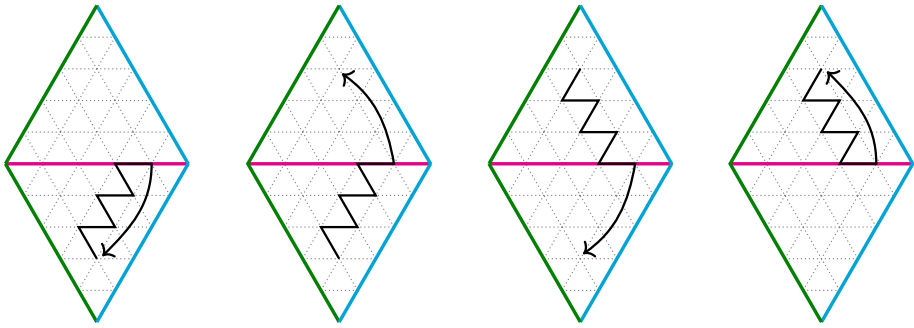
Fig. 24 The first (respectively last) two paths are S_\alpha and P_\alpha^b originating in an alcove with \alpha labelling an upper (respectively lower) wall. Here we take the convention that the origin is below the pink hyperplane. The degrees of these paths are 1, 0, 0, -1 respectively. We call these paths U_0, U_1, D_0, and D_1 respectively
