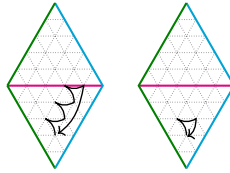
Fig. 21 We let h = 3, \ell = 1, e = 5 and \alpha = \varepsilon_3 - \varepsilon_1 and we depict the paths P_\alpha^b and P_\emptyset (we actually only depict P_\emptyset which is a third of the path P_\emptyset ). We have already constructed the corresponding element \text{spot}_\alpha^\emptyset in great detail over the course of Examples 3.6, 3.8 and 3.10 and Fig. 13
