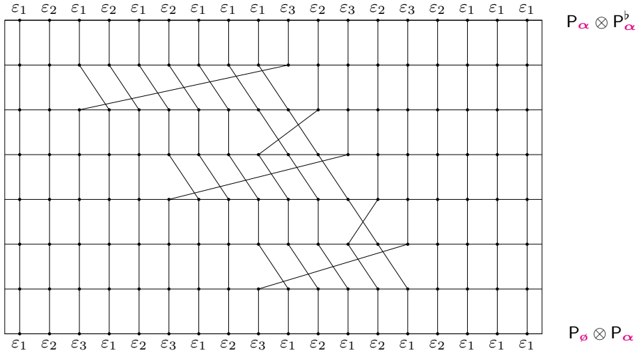
Fig. 22 Fix \ell = 1 and h = 3 and e = 5 and \alpha = \varepsilon_3 - \varepsilon_1 (so that b_\alpha = 3 ). We picture the element \Upsilon_{P_\emptyset \otimes P_\alpha}^{P_\alpha \otimes P_\alpha^b} . The first 9 and final 4 of the branching coefficients are trivial and so we do not waste trees by picturing all of them. The corresponding paths are pictured in Fig. 23
