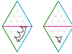
Fig. 21 We let h = 3, \ell = 1, e = 5 and \alpha = \varepsilon_3 - \varepsilon_1 and we depict the paths P_\alpha^b and P_\emptyset (we actually only depict P_\emptyset which is a third of the path P_\emptyset ). We have already constructed the corresponding element \text{spot}_\alpha^\emptyset in great detail over the course of Examples 3.6, 3.8 and 3.10 and Fig. 13
