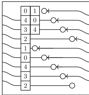
Fig. 4 For n = 13 and \lambda = (2^3, 1^6) , we illustrate how the idempotent, e_{(0,1,4,0,3,4,2,1,0,4,3,2,2)} , labelled by J in Fig. 3 is rewritten in the form (2.8). The box moves through each row until it comes to rest at the point J^{-1}(13) = [1, 3, 0] . This involves repeated applications of Eq. (2.6) to deduce (2.8). For the purposes of later referencing, we label the 9 boxes from bottom-to-top by \alpha_1 = [9, 6, 0], \alpha_2 = [8, 5, 0], \dots, \alpha_9 = [1, 3, 0] . This visualisation is explained in Remark 2.18
