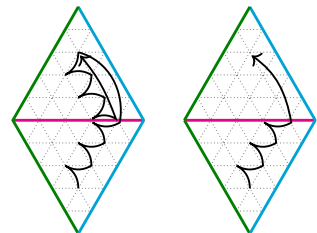
Fig. 22 Fix \ell = 1 and h = 3 and e = 5 and \alpha = \varepsilon_3 - \varepsilon_1 (so that b_\alpha = 3 ). We picture the element \Upsilon_{P_\emptyset \otimes P_\alpha}^{P_\alpha \otimes P_\alpha^b} . The first 9 and final 4 of the branching coefficients are trivial and so we do not waste trees by picturing all of them. The corresponding paths are pictured in Fig. 23
