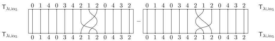
Fig. 9 The righthand-side of Eq. (2.18) for \lambda = (2^6, 1^3) and \alpha_5 as in Fig. 4. The left diagram factors through the element y_{T_{\lambda \cup \alpha_6}}^{\tilde{\lambda}} ; we will further manipulate this in Fig. 10 below
