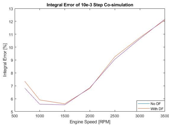
Figure 10. Angular impulse percent error vs. engine speed
