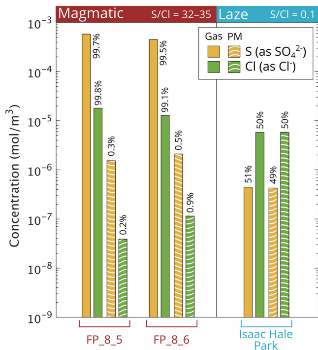
Fig. 3 S and Cl in the magmatic and laze plumes. Concentrations ( \text{mol}/\text{m}^3 ) of S (measured as \text{SO}_4^{2-} ) and Cl (measured as \text{Cl}^- ) in the gas and PM phases of the magmatic (left, two unsaturated ground samples) and laze plumes (right, unsaturated Isaac Hale Park sample). Percentages indicate the proportion of S and Cl measured as gas and PM for each element. S/Cl ratios are total (gas + PM) molar ratios. Cl in PM at Fissure 8 is comparable to background levels measured in 2019 16 (Supplementary Data 1 Table S7). Errors are \pm 33\% for \text{Cl}^- and \pm 35\% \text{SO}_4^{2-} . Data and propagated errors can be found in Supplementary Data 1 Tables S7 and S11 for the magmatic and laze plumes, respectively.
