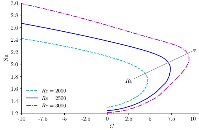
Figure 13: Continuation in C from N4L for increasing values of Re . The curve for Re = 2500 is the same as that shown in figure 10(right).
