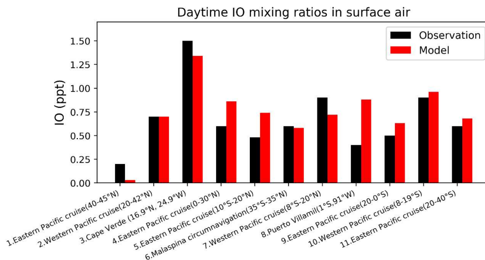
Figure 10. Daytime surface air mixing ratios of IO from island sites and ocean cruises, arranged from left to right in order of decreasing latitude. Observed values (black) are means for the reporting period in different years. Model values (red) are monthly mean values in 2016 taken for the same month and location as the observations. References: (1,4,9,12) Mahajan et al. (2012); (2,7,10) Großmann et al. (2013); (3) Mahajan et al. (2010); (5) Volkamer et al. (2015); (6) Prados-Roman et al. (2015); (8) Gómez Martín et al. (2013).
