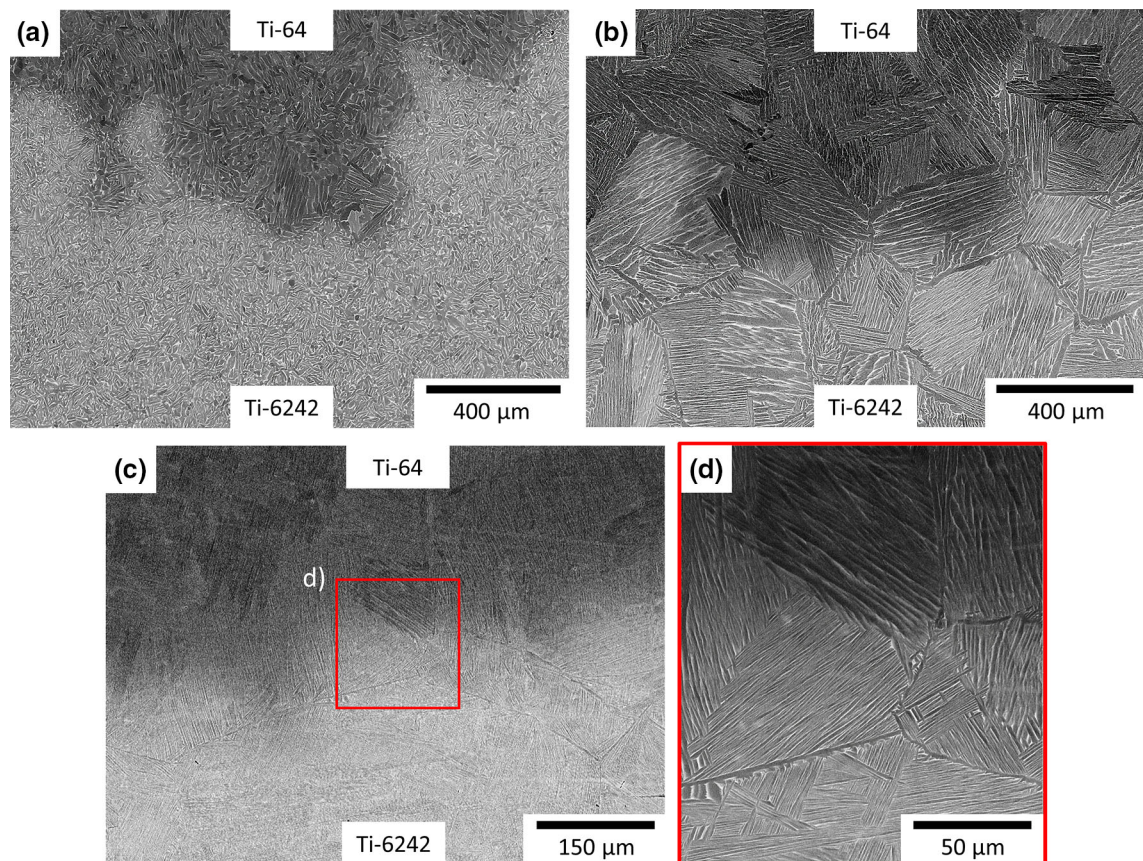
Fig. 5—Backscatter electron images of the FAST-DB sample processed under (a) subtransus conditions (TDB1), (b) supertransus conditions (TDB2), (c) supertransus conditions (TDIC), (d) supertransus conditions (TDIC) at higher magnification.
