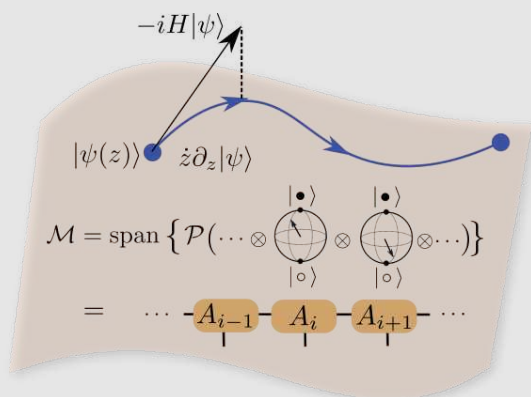
Figure B2 | Variational method for quantum many-body scars. Time-dependent variational principle captures the optimal projection of quantum dynamics onto a given variational manifold. The studies of PXP model use matrix product states (MPS) as a variational manifold, where each atom is described by a single angle. The presence of the Rydberg blockade, implemented by projector \mathcal{P} , results in entanglement, which requires a bond dimension 2 of MPS tensors, A_i .
