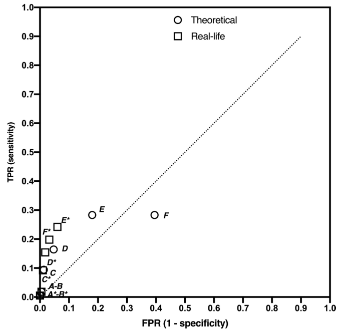
Figure 3 Sensitivity and specificity of combinations of HIA1 assessment subtests with and without clinical judgement applied. The theoretical TPR and FPR are indicated by circles, while real-life TPR and FPR are shown as square symbols. key: (A) all modes abnormal, (B) five modes abnormal, (C) four modes abnormal, (D) three modes abnormal, (E) two modes abnormal, (F) single mode abnormal. FPR, false positive rate; TPR, true positive rate.
