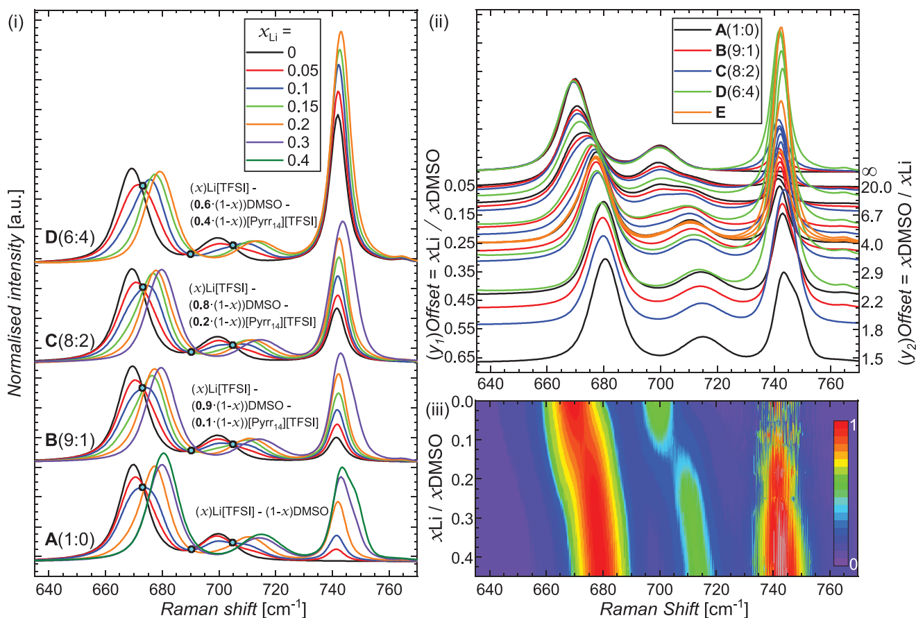
Figure 5. Raman spectra for ternary Li[TFSI]:DMSO:IL formulations. i) Spectra grouped by x_{DMSO}:x_{[Pyrr_{14}][TFSI]} ratios, ii) spectra stack plotted, and iii) intensity heat maps of all spectra, wherein the y -axis offset is proportional to the critical ratios between DMSO and Li[TFSI]. The color map in (iii) is scaled with respect to the intensity of \delta_s(C-S) in pure DMSO. Isosbestic points in more dilute formulations (where free DMSO is observed) are shown by the blue circles at 673, 689, and 705 cm^{-1} .
