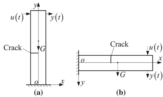
Fig. 5 Experimental setup for detection of cracks in beams. a Vertical setup; b Horizontal setup
