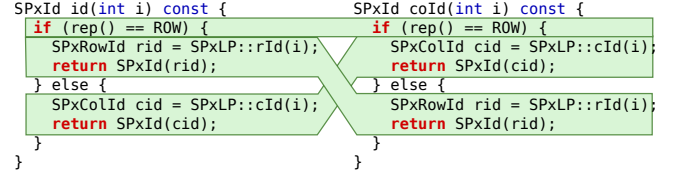
Figure 4. Example with code reordering extracted from the 450.soplex program.
