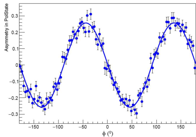
Fig. 5 Visualisation of asymmetry constructed from extracted \Sigma values as defined in Eq. 8. Blue points are the data and blue solid line is the result of the maximum likelihood fit
