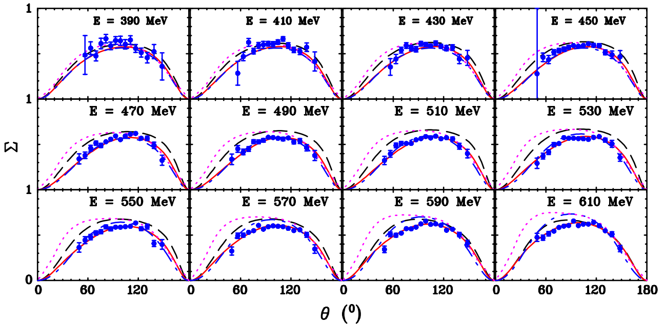
Fig. 6 \Sigma for \vec{\pi}n \rightarrow \pi^0 n vs. pion production angle \theta in c.m. frame: A2 (blue filled circles); fit: SAID MU22 (red solid curves), SAID MA19 [4] (blue dash-dotted curves), Bonn-Gatchina BG2014-02 [28] (magenta dotted curves), and MAID2007 [29] (black dashed curves). Only angle-dependent uncertainties are shown for all data. Each plot corresponds to a 20 MeV wide bin in E_\gamma with the central value given in each.
