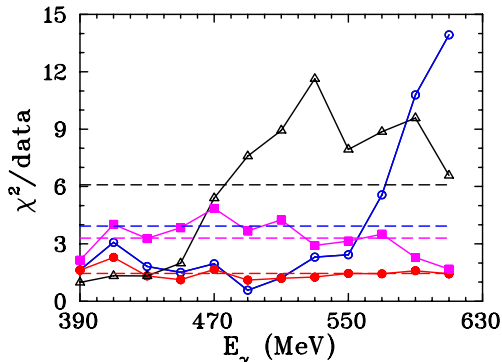
Fig. 7 Comparison of \chi^2 per data point for the previous SAID solution MA19 [4] and MAID2007 [29] applied to the present A2 data with blue open circles and black open triangles, respectively. The new SAID solution MU22 (MUXX) with red full circles and magenta full squares obtained after adding the present A2 data (MUXX does not have any \gamma n \rightarrow \pi^0 n data). Also shown are the fit \chi^2 per data point values averaged over each energy bin E_\gamma , where the horizontal dashed lines are for the MU22 (red), MUXX (magenta), MA19 (blue), and MAID2007 (black) solutions. The solid lines connecting the points are included only to guide the eye.
