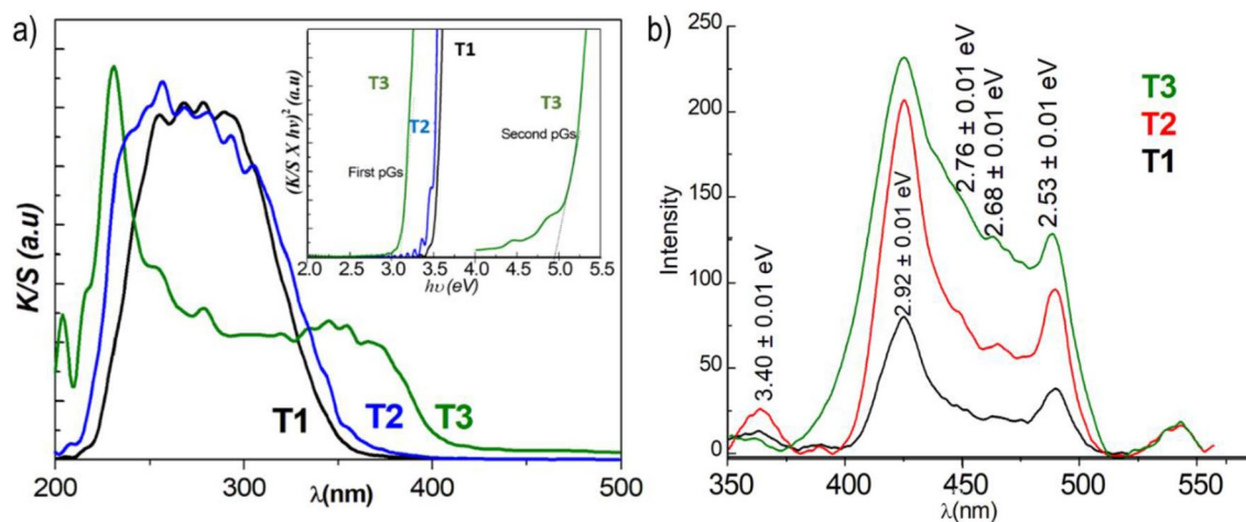
Figure 12. Reflectance diffuse spectra (after Kubelka–Mulk transformation) 93 of T1, T2, and T3 lamellar \text{H}_2\text{Ti}_3\text{O}_7 NTs, and (inset) plot (K/S \times hv)^2 against h\nu showing the linear fitting to the main linear segment of the curve considering a direct band gap transition, according to the Tauc equation (a). Luminescence emission spectra of T1, T2, and T3 (b).
