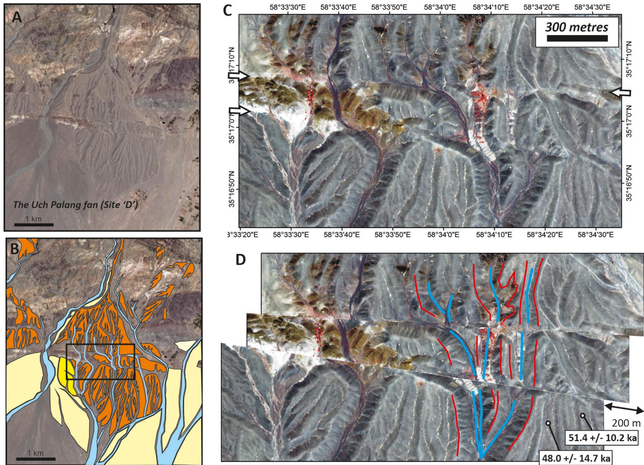
Figure 13. (a) The Uch Palang alluvial fan (Site D). (b) Geomorphic interpretation of the site. The oldest fan surface is in orange and the youngest surface in pale yellow. The small surface shown in bright yellow may be intermediate in age. (c) Close up IKONOS image showing the fault crossing the older fan surface. (d) Restoration of 200 \pm 50 m restores the drainage channels (channel bases in blue and tops in red) to their original linear shape. Ages from Fattahi et al. (2007) are shown.
