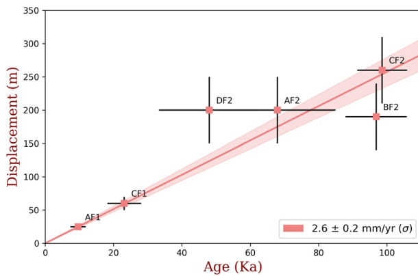
Figure 14. Plot of age against displacement for the dated landforms, with each labeled by site and then fan generation (i.e., DF2 = Site D, fan F2). An orthogonal distance regression is fitted to the six data points for which we have reliable age and displacement measurements (these six measurements are shown as red squares, with their uncertainties shown as black bars). The regression takes into account the uncertainties in both age and distance uncertainties (one-sigma for both). The best fit line is shown in red, with two-sigma uncertainty in the regression represented by the pink area. In the plot shown, the best fit line is constrained to pass through the origin. If the best fit line is not constrained to pass through the origin the mean slip-rate does not change, but the uncertainty increases from \pm 0.2 to \pm 0.3 mm/yr.
