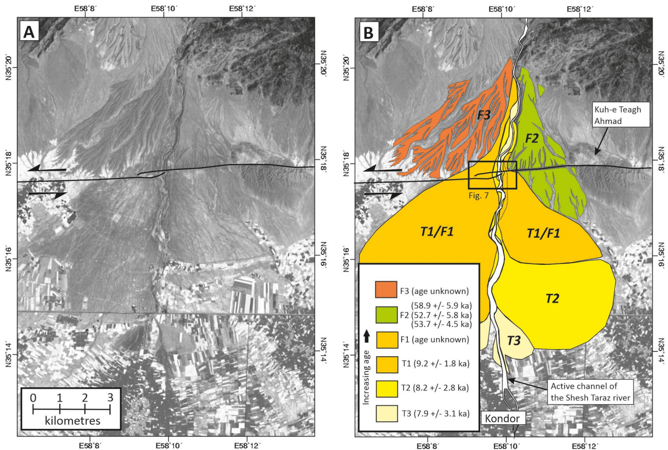
Figure 6. (a) ASTER image of the Shesh-Taraz river. The Doruneh fault cuts east-west across the center of the image, forming a small pull-apart immediately west of the main river channel. (b) The same image with interpretation of the geomorphology, along with available age constraints (see text for details). Three main alluvial fan surfaces are recognized on the basis of elevation and level of incision. They are labeled F1–F3, from youngest to oldest. Fluvial terraces inset into the F1 surface are labeled T1–T3. The uppermost fluvial terrace is separated from the surface of fan F1 by a small riser (see Figure 7). T1 and F1 merge downstream to form a single fan, which we label T1/F1. T2 and T3 correspond to alluvial fans formed in the basin interior. The present-day river channel is incised until the village of Kondor, far south of the Doruneh fault. The box represents the area shown in Figure 7.
