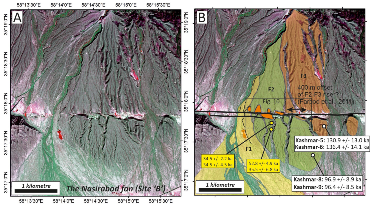
Figure 9. (a) Quickbird imagery of an alluvial fan complex near Nasirabad village “Site B.” (b) An interpretation of the geomorphology, along with available age control (white—this paper; yellow—Farbod et al., 2016). Three main fan surfaces are identified, and shaded in yellow, green, and orange from youngest to oldest. Small hills formed of older alluvium are colored in opaque orange.
