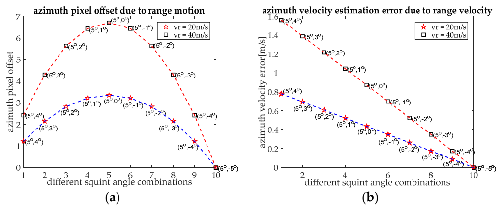
Figure 4. The effect of range velocity on azimuth velocity estimation with v_r = 20\text{m/s} and v_r = 40\text{m/s} : (a) Azimuth pixel offset is positively related to the difference in the absolute value of squint angles; (b) Azimuth velocity estimation error is negatively related to the difference of the angles.
