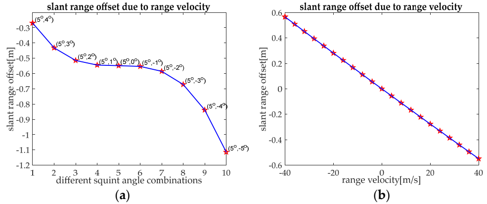
Figure 5. Slant range offset caused by range motion among sequential SAR images: (a) With v_r = 40 \text{ m/s} , v_a = 0 and this offset is positively related to deviation of the angles; (b) with squint angle combination (5^\circ, 0) .
