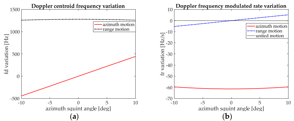
Figure 3. Doppler spectrum shift with v_a = 40\text{ m/s} and v_r = 40\text{ m/s} : (a) Range velocity leads to a basically symmetric f_d variation and azimuth velocity leads to a basically linear variation; (b) Range velocity leads to a basically linear f_r variation and azimuth velocity leads to a basically symmetric variation.
