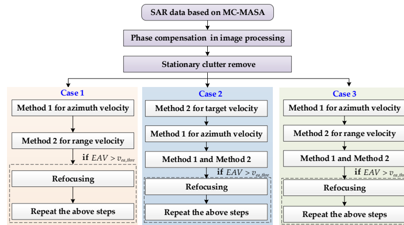
Figure 7. Flowchart of the proposed velocity estimation method.
