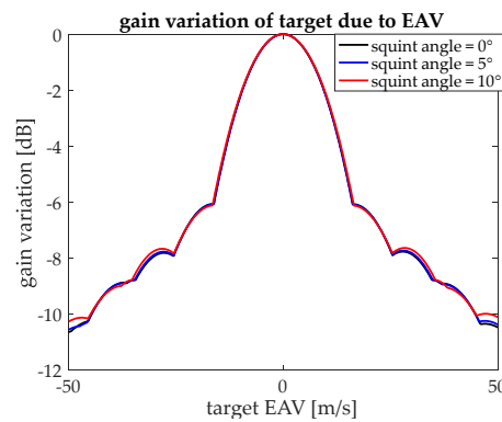
Figure 6. Gain variation of target caused by EAV. For isotropic target, gain variation is dependent on EAV and independent of squint angles.
