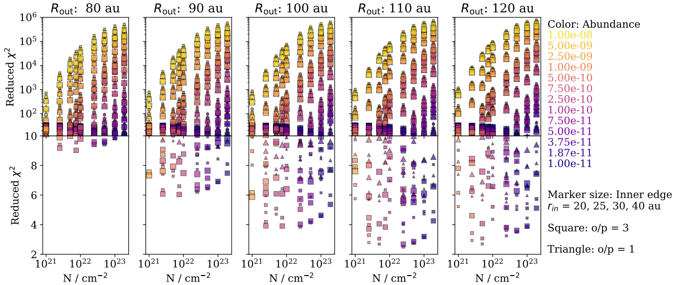
Figure 4. Reduced \chi^2 between the observed visibilities and modelled visibilities. Each point represents the model fit for all observed lines as a summed reduced \chi^2 . The model parameters are described by the point color (abundance), size (inner radius of c\text{-C}_3\text{H}_2 ), and shape (ortho to para ratio). The columns indicate different outer radii for the c\text{-C}_3\text{H}_2 slab, for the full range of \text{H}_2 column densities considered on each x-axis. The poor fits are shown on a logarithmic scale on the top row, while the better fits are shown as a linear scale on the bottom row.
