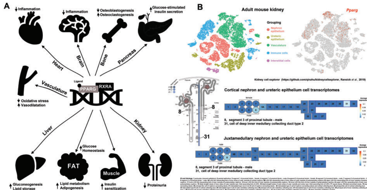
FIGURE 1: (A) TZDs activate PPAR \gamma -retinoid X receptor functional heterodimers, which in turn regulate gene transcription (PPAR response elements) in multiple tissues, resulting in widespread effects on metabolism, osteogenesis, proteinuria, vascular reactivity and inflammation as reviewed by Mao and Ong [4]. (B) Single-cell Pparg gene expression in mouse adult kidney showing predominant expression in the vasculature and immune cells with detectable low tubular expression in specific segments, i.e. S3 proximal tubule and inner medullary collecting duct (average expression <0.04). The numbered segments correspond to the segmentation reported in the Kidney Cell Explorer (Ontology identification 1–32) [11].
