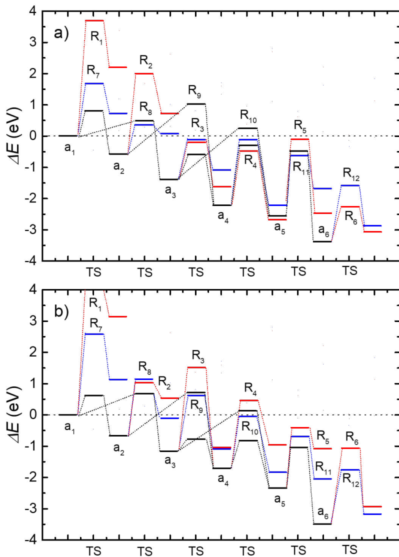
FIG. 4. Energy profile for (black line) the reduction mechanism of \text{CHO}-\text{CHOO} to \text{CH}_3-\text{COOH} on the (a) \text{Fe}_A and (b) \text{Fe}_B sites of the \text{Fe}_3\text{S}_4\{111\} surface; alongside the competitive (red line) non-promoted and (blue line) H-promoted elimination of OH and \text{H}_2\text{O} , respectively. Intermediates and reaction labels are provided according to Tables 1-3.
