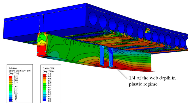
Figure 8. Final configuration for W360x51, f_c = 25 MPa, \varphi = 10 mm, and 120 mm of spacing.
