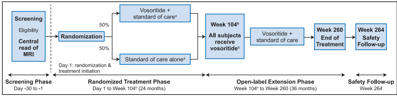
Figure 1. Study design.
