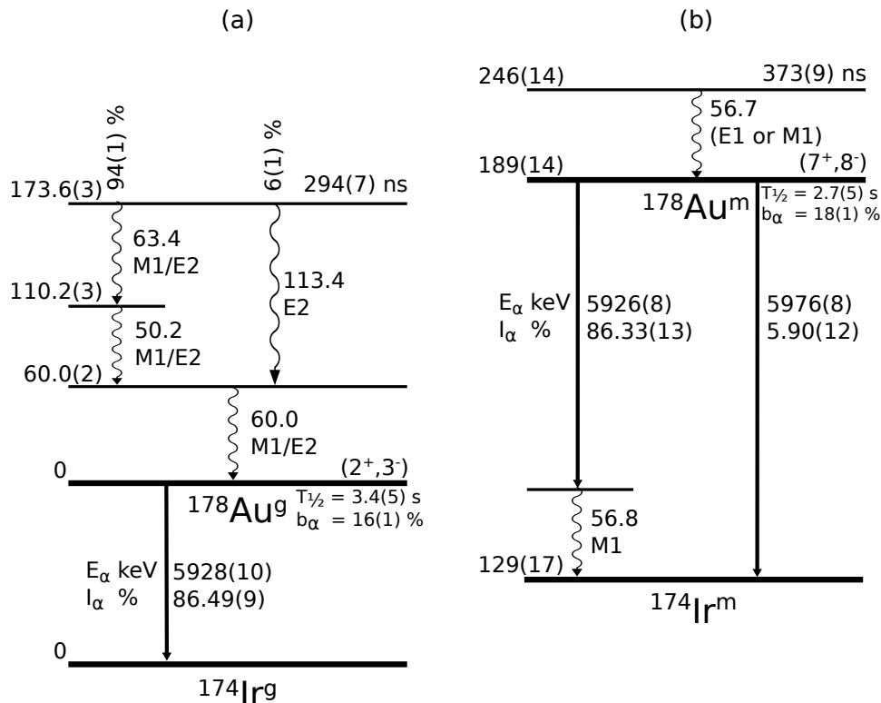
FIG. 4. (a) Proposed decay schemes of the new 294-ns isomeric state in ^{178}\text{Au} , de-exciting to the low-spin ^{178}\text{Au}^g \alpha/\beta -decaying state. (b) Decay scheme of the new 373-ns isomeric state de-exciting to the high-spin ^{178}\text{Au}^m \alpha/\beta -decaying state. The quoted \alpha -decay energies are from the present work, while the half-lives, \alpha -decay branching ratios, relative intensities of \alpha decays and relative energies for ^{178}\text{Au}^{m,g} are from [18]. Only selected alpha decays relevant to this work and observed in our study are shown here, for the full \alpha -decay and intensities of all other (weaker) \alpha decays, see [18].
