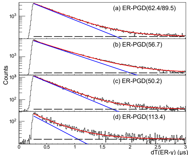
FIG. 3. (color online) (a) Decay curve for the sum of data for the 62.4- and 89.5-keV transitions in ^{179}\text{Au} . The fit (in red) consists of an exponential function (in blue) and a constant background (dashed black); (b) same as (a), but for the 56.7 keV transition in ^{178}\text{Au} ; (c) same, but for the 50.2 keV transition in ^{178}\text{Au} ; (d) same, but for the 113.4 keV transition in ^{178}\text{Au} .
