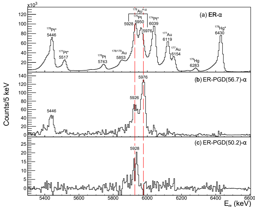
FIG. 1. (color online) (a): Energy spectrum of \alpha decays, observed within 7 s of ER implantation in the DSSD. Peaks are labelled with their energies, in keV, and with the isotope, they originate from. An asterisk marks the peaks used to calibrate the DSSD; (b) Same as (a), but a 56.7 ( \pm 1.0 -keV energy window) \gamma decay must also be detected in the PGD within the time of \Delta T(\text{ER-PGD}) = 0\text{--}1 \mu\text{s} ; (c) Same time gates as (b), but with an energy gate on the 50.2 ( \pm 1.0 -keV energy window) keV transition in the PGD.
