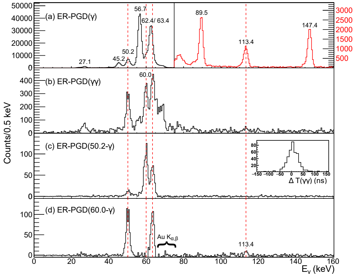
FIG. 2. (a) Recoil-gated singles \gamma -ray spectrum, observed in the PGD within the time of \Delta T(\text{ER-PGD}) = 0\text{--}1 \mu\text{s} of the ER implantation in the DSSD. The centroids of the peaks are obtained from fits and labelled with their energies in keV. Note the change of the Y-axis scale from 80-keV on; (b) Projection of a recoil-gated PGD( \gamma\gamma ) matrix for events with the prompt time condition \Delta t(\gamma\text{--}\gamma) \leq 70 \text{ ns} ; (c) same as (b), but with an energy gate of \pm 1 \text{ keV} applied on the 50.2-keV transition; (d) same time gates as (c), but with an energy gate of \pm 1 \text{ keV} on the 60.0-keV transition. The inset to (c) shows the time distribution for the 50.2–63.4-keV coincident events.
