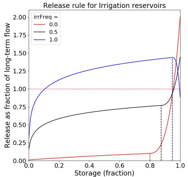
Figure 4. Impact of the seasonal shape parameter on reservoirs whose primary purpose is irrigation. Dashed lines indicate the inflection point S^* . We have \text{irrFreq} = 1 between 18 July and 30 August included, 0 between 12 October and 23 April included and 0.5 during the shoulder seasons.
