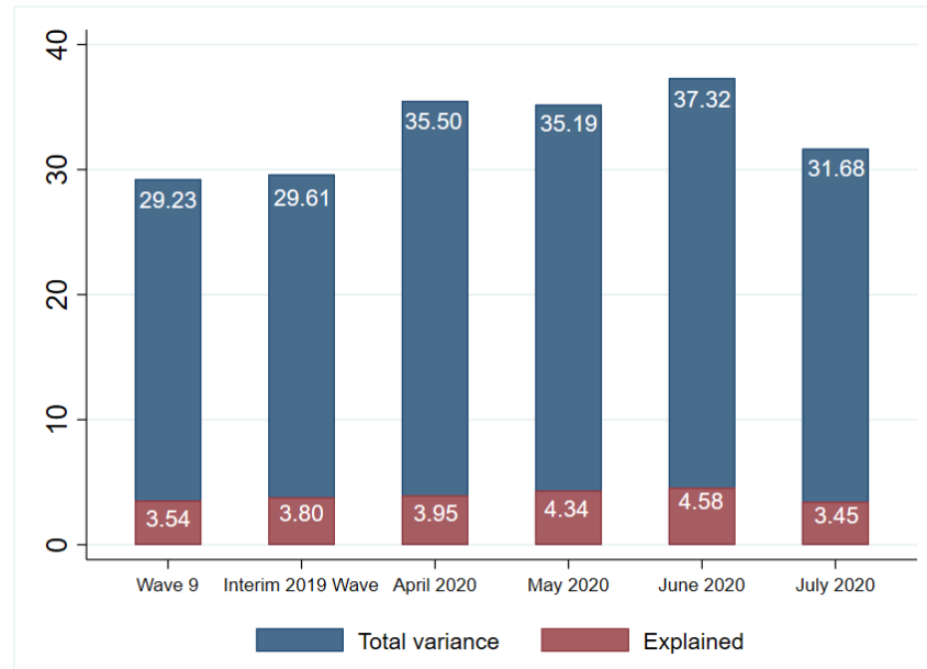
Figure 2: Total and explained variance of GHQ-12 Likert score.
