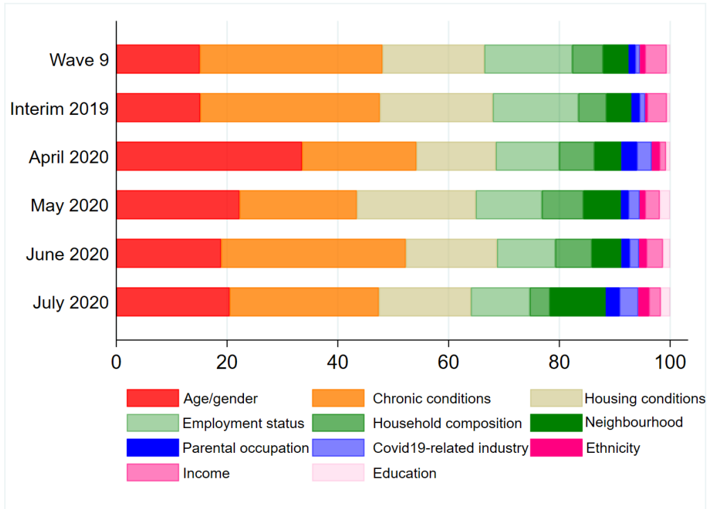
Figure 3: Decomposition analysis of GHQ-12 Likert scores.
