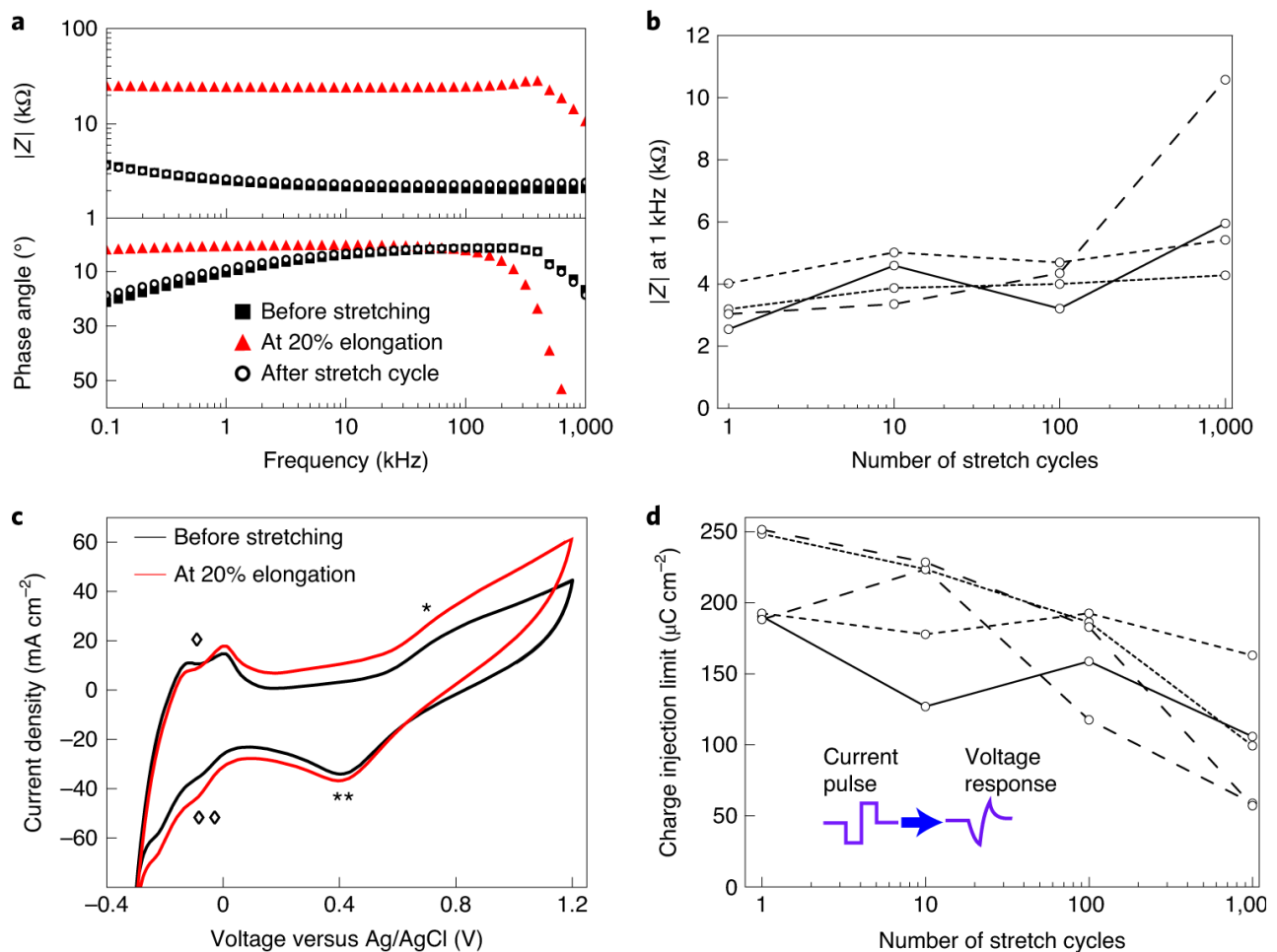
Fig. 3 | Electromechanical properties.
