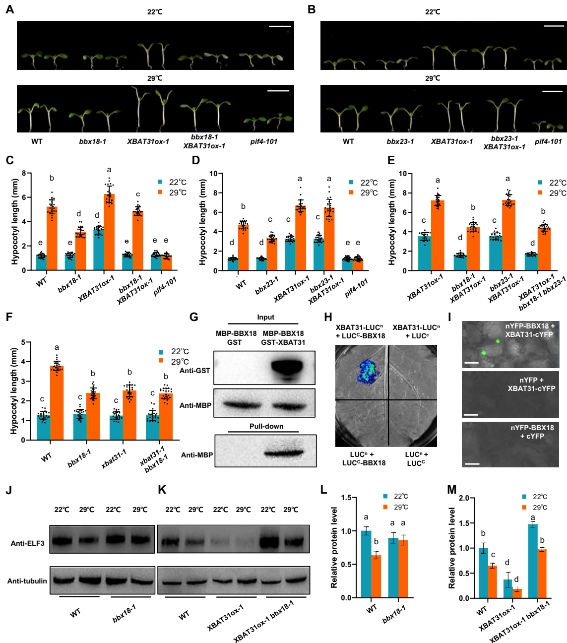
Fig. 5. XBAT31-mediated ELF3 degradation is dependent on BBX18. (A to F) Requirement of BBX18 for XBAT31 -mediated thermomorphogenesis. XBAT31 overexpression plant ( XBAT31ox-1 and WT background) was crossed to the bbx18-1 , bbx23-1 , or bbx18-1 bbx23-1 mutant. xbat31-1 was also crossed to bbx18-1 . Seedlings grown at 22°C were transferred to either 22° or 29°C for 4 days, after which representative plants were imaged (A and B). The hypocotyl length was subsequently measured (C to F). Error bars depict SD ( n = 24 ). Scale bars, 5 mm. (G to I) Protein-protein interaction between XBAT31 and BBX18 in the pull-down assay (G), split-luciferase assay (H), and split-YFP assay (I). MBP-BBX18 and GST-XBAT31 were incubated and immunoprecipitated with Glutathione-Superflow resins and detected using anti-MBP antibody (G). Different combinations of constructs were agro-infiltrated into tobacco leaves, and the chemiluminescence or fluorescence was detected (H and I). Empty vectors were used as controls. Scale bars, 50 \mu\text{m} . (J to M) Dependence of BBX18 for the XBAT31 -regulated ELF3 stability. WT, bbx18-1 mutant, XBAT31ox-1 , or XBAT31ox-1 bbx18-1 plants grown at 22°C were transferred to 29°C, and ELF3 was checked with an anti-ELF3 antibody (J and K) and quantified (L and M). Tubulin was used as a loading control. Error bars represent SE ( n = 3 ). Letters above the bars indicate significant differences as determined by post hoc test ( P < 0.05 ).
