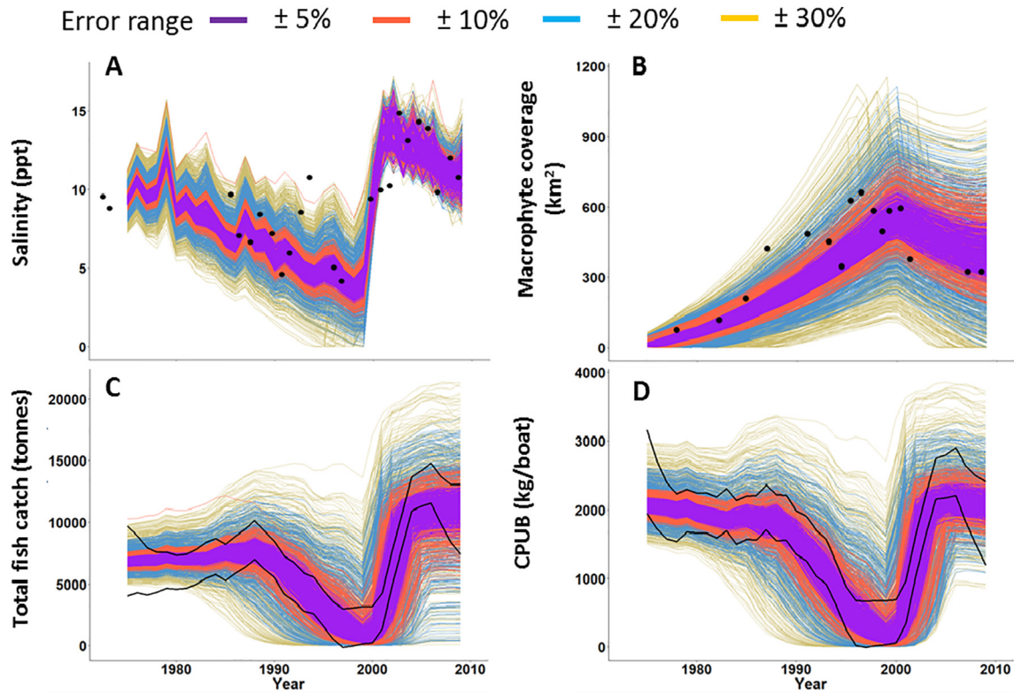
Fig. 3. Graphical outputs from the second stage of generalised sensitivity analysis where the six critically sensitive variables (Table 1) are simulated under four error ranges; 500 simulations are run per error range. Observations (black) are plotted against model generated time-series of four social-ecological processes: (A) salinity; (B) aquatic vegetation coverage; (C) catch (99% confidence intervals in black) (D) catch per unit boat (99% confidence intervals in black).
