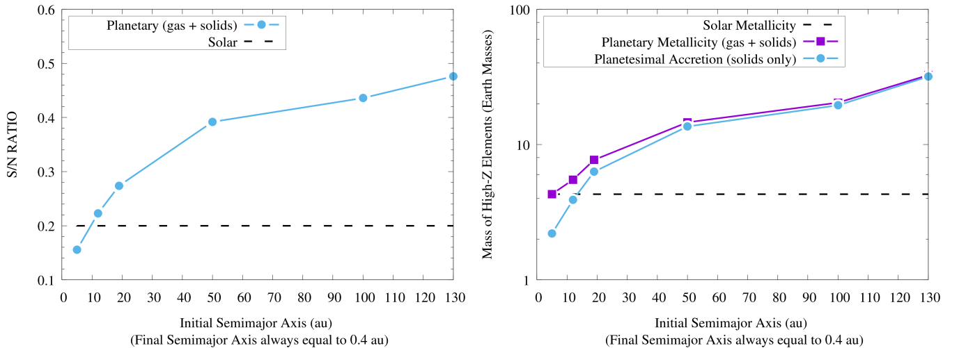
Figure 6. S/N ratio ( left ), metallicity and mass of accreted planetesimals ( right ) of solid-enriched giant planets as a function of their initial orbital positions. The dashed lines show the stellar S/N ratio and the mass of high- Z elements equivalent to the stellar metallicity, which are the same as the solar ones. We refer the readers to Sect. 3.4 for details.
