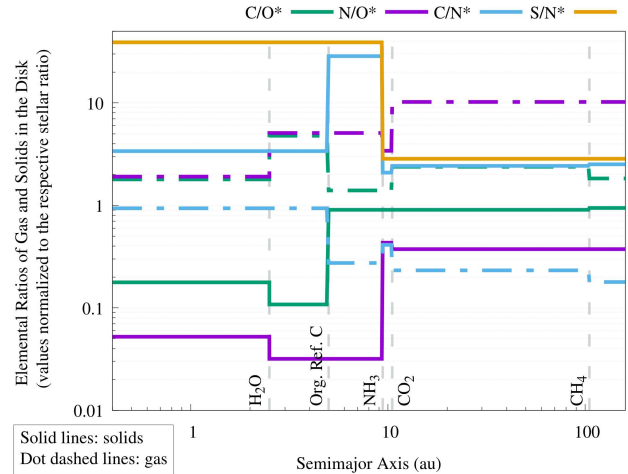
Figure 9. Elemental ratios of the gas (dot-dashed lines) and the solids (solid lines) in the protoplanetary disk as a function of the radial distance from the star. Each elemental ratio is normalized to the relevant stellar elemental ratio.
