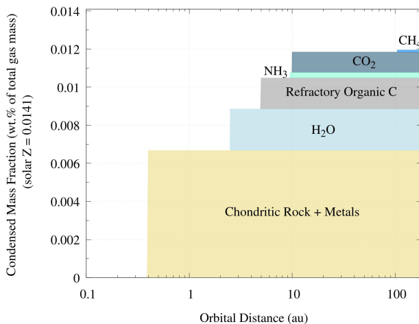
Figure 2. Mass fraction of solid material as a function of the distance from the star in our template protoplanetary disk. The mass fraction is expressed with respect to the total mass of gas assuming a solar composition for the latter. The mass fraction of condensed material is always lower than the protostellar Z as some elements (Ne) and molecules (CO and N 2 ) never condense in our disk (see main text and Table 3 for further details).
