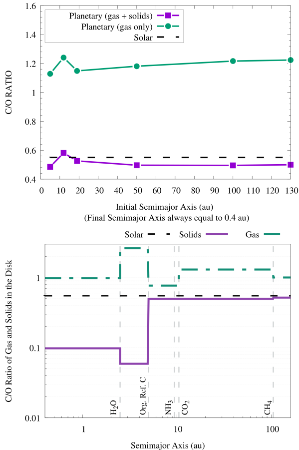
Figure 4. Top: Final C/O ratios of the gaseous envelope of the giant planet as a function of its initial orbital position for the
