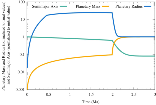
Figure 1. Normalized growth and migration tracks from the scenario where the giant planet starts forming at 5 au. The growth tracks of both mass and radius are normalized to the final mass ( 1 M_J ) and radius ( 1.6 R_J ) of the giant planet. The migration track is instead normalized to the initial semimajor axis (5 au) of the giant planet.
