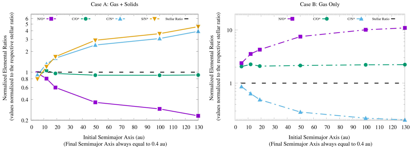
Figure 8. Same as Fig. 7 but assuming a 9:2 \text{N}_2:\text{NH}_3 ratio instead of the 1:1 ratio from Eistrup et al. (2016, 2018) adopted in our standard compositional model. The contrast among the different elemental ratios in the solid-enriched metallicity case is enhanced by a factor of two, while the effects of this alternative partitioning are more limited in the gas-dominated metallicity case.
