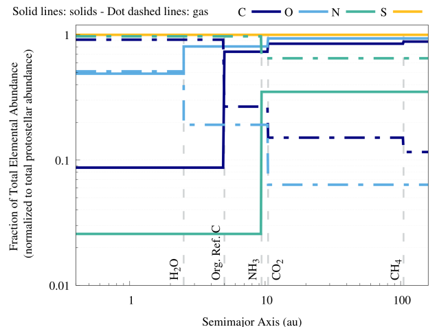
Figure 3. Fractions of C, O, N and S in solid phase (solid lines) and gas phase (dot dashed lines) in the protoplanetary disk at varying distances from the host star. The values are normalized to the protostellar abundances reported in Tables 1 and 2. The vertical dashed lines indicate the position of the snowlines of H 2 O (2.5 au), refractory organic carbon (5 au), NH 3 (9.4 au), CO 2 (10.5 au) and CH 4 (105 au).
