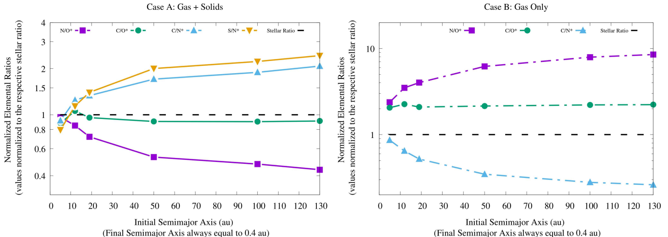
Figure 7. Left: normalized elemental ratios of the gaseous envelope when the metallicity of the giant planet is dominated by the accretion of planetesimals. Right: normalized elemental ratios in the gaseous envelope when the metallicity of the giant planet is dominated instead by the accretion of gas. Each elemental ratio is normalized to the relevant stellar elemental ratio.
