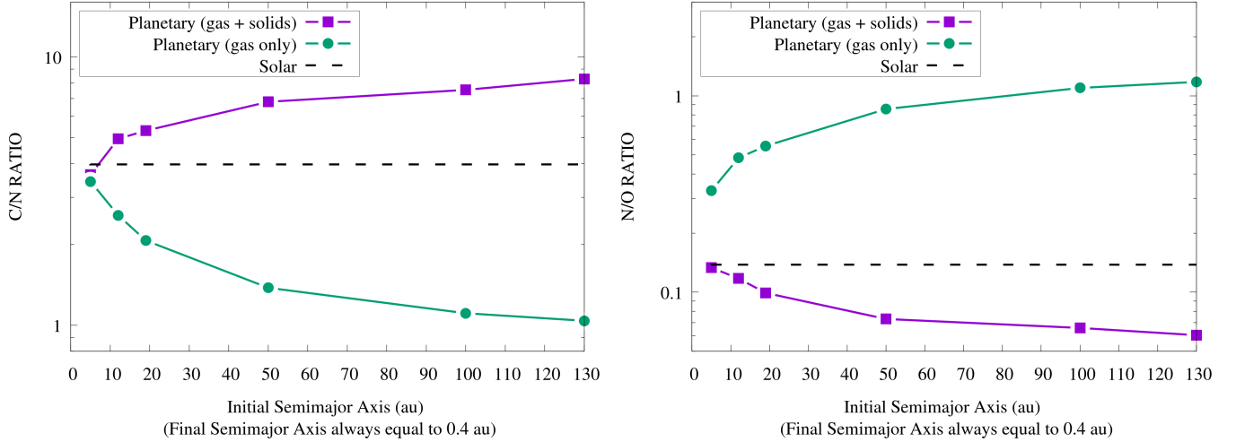
Figure 5. C/N ( left ) and N/O ( right ) ratios of the gaseous envelope of the giant planet as a function of its initial orbital position. In the figure we show the cases of solid-enriched giant planets (purple line and squares) and gas-dominated giant planets (green line and circles). The dashed lines show the stellar C/N and N/O ratios, which are the same as the solar ones. We refer the readers to Sect. 3.3 for details.
