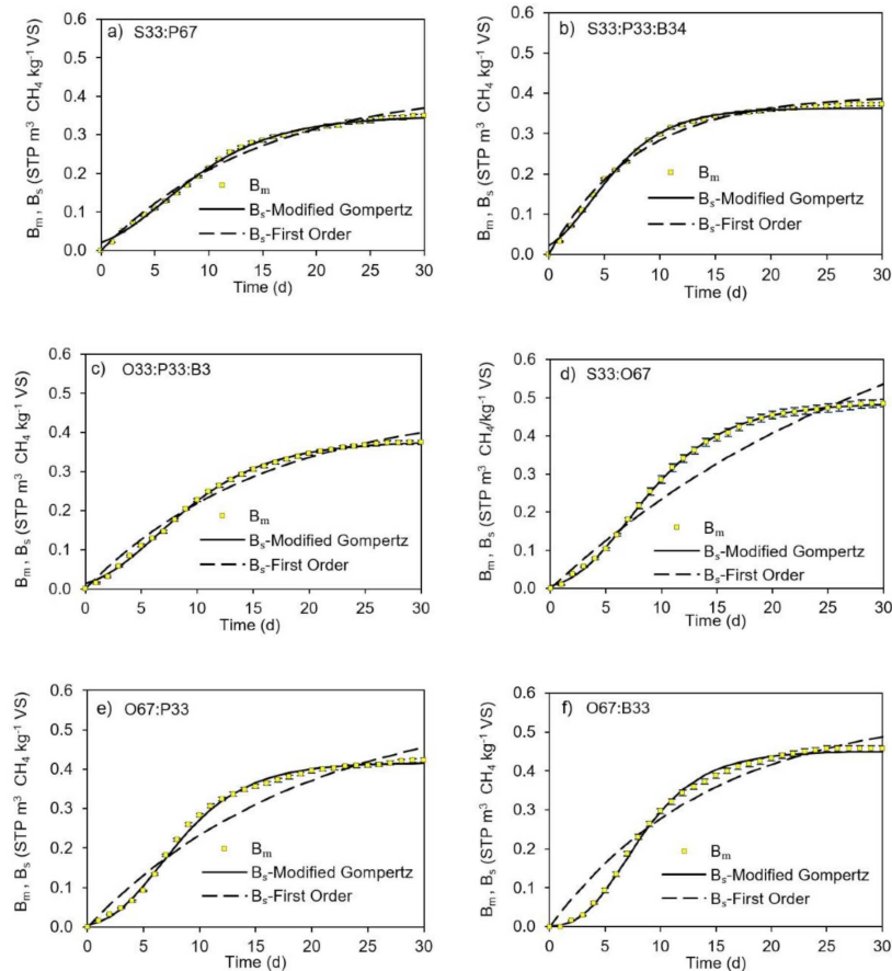
Figure 4. Accumulative CH 4 production from experimental data (B m ) and calibrated model (B s ) of the mixtures with the smallest deviations (a–c) and the greatest deviations (d–f) from the first-order model. The letter represents the waste stream (S: slaughter wastewater; O: offal wastewater; P: paunch wastewater; B: bovine manure) and the number its %VS in the mixture.
