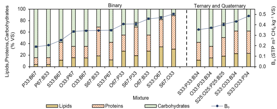
Figure 3. Biochemical composition of the different AcoD mixtures (left axis) and the resulting ultimate specific CH 4 yield (right axis). On the X-axis, the letter represents the waste stream (S: slaughter wastewater; O: offal wastewater; P: paunch wastewater; B: bovine manure) and the number its %VS in the mixture.
