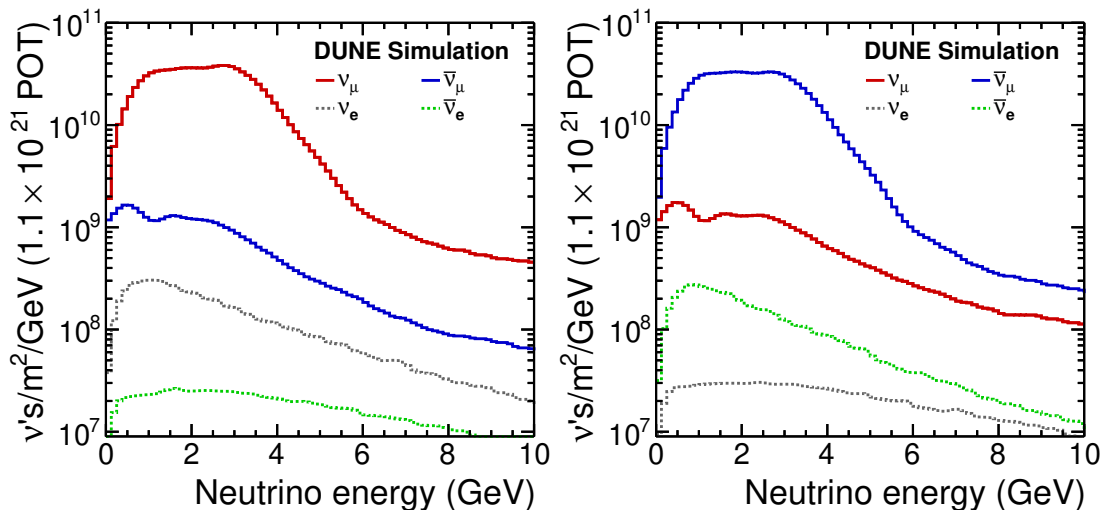
FIG. 2. Unoscillated neutrino fluxes at the far detector for neutrino-enhanced, FHC, beam running (left) and antineutrino, RHC, beam running (right). Figure reproduced from [2].
