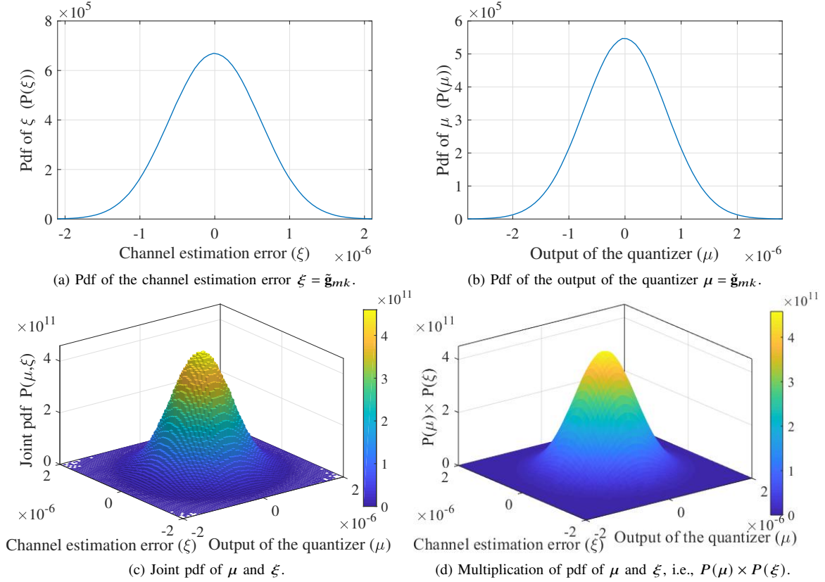
Figure 11. Pdf of \mu = \check{\mathbf{g}}_{mk} and \xi = \hat{\mathbf{g}}_{mk} with \alpha = 1 quantization bit.
