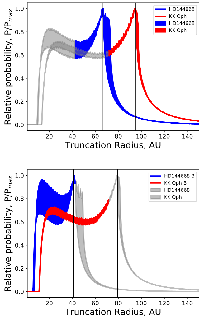
Figure 4. Normalised probability distributions of the truncation radius of the primary (upper panel) and secondary (lower panel) discs of HD 144668 (blue) and KK Oph (red). The primaries are resolved, but the secondaries are not, which allows us to place constraints on the disc size relative to that of the beam. This places lower limits on the primary disc sizes (denoted by the gray shaded region, which goes up to the beam size) and upper limits on the secondary disc sizes (again, denoted by the gray region in the lower panel, which is beyond the beam size). The vertical lines denote the peak probabilities.
