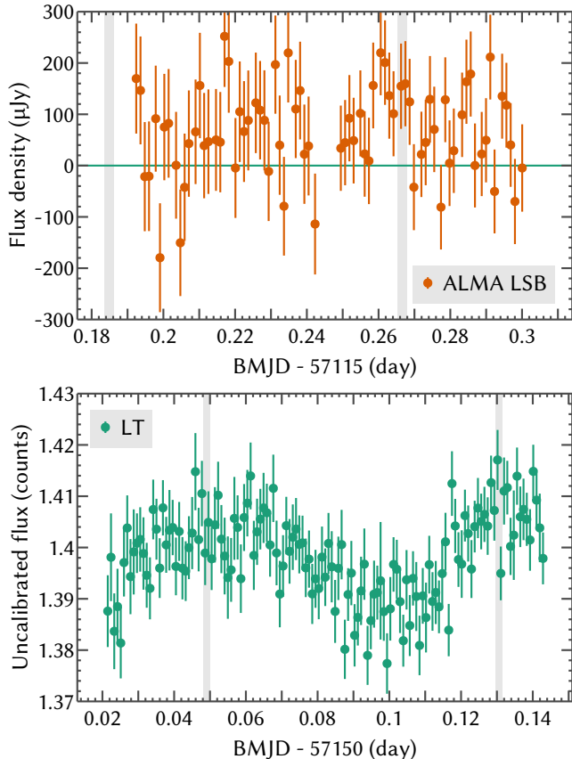
Figure 2. Light curves of TVLM 513 in millimeter (ALMA LSB; upper panel) and optical (lower panel) bands. The sampling intervals are 102 and 78 seconds, respectively. Both panels have widths of 3.31 hr. The vertical gray bands indicate the 1\sigma confidence bounds on the time of optical maximum as derived empirically from the LT data and propagated assuming a period of 1.95958 \pm 0.00005 hr (Harding et al. 2013). The ALMA observations occurred 426 rotations prior to the LT observations. The possible increase in millimeter emission at BMJD 57115.265 occurs at the time of optical maximum.
