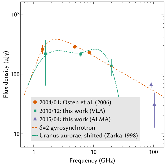
Figure 3. Non-simultaneous centimeter-to-millimeter spectrum of TVLM 513. The orange points show the data obtained quasi-simultaneously by Osten et al. (2006); green show the quasi-simultaneous VLA data described in Section 3.2; blue show the simultaneous ALMA data described in Section 3.1. The dashed lines show two representative spectral models described in Section 4.2; they disregard the long time baseline between the relevant VLA and ALMA observations and should not be used for quantitative analysis.
