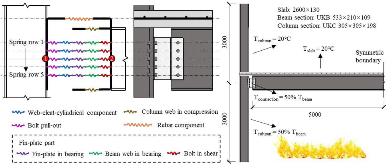
(a) The proposed component-based model
